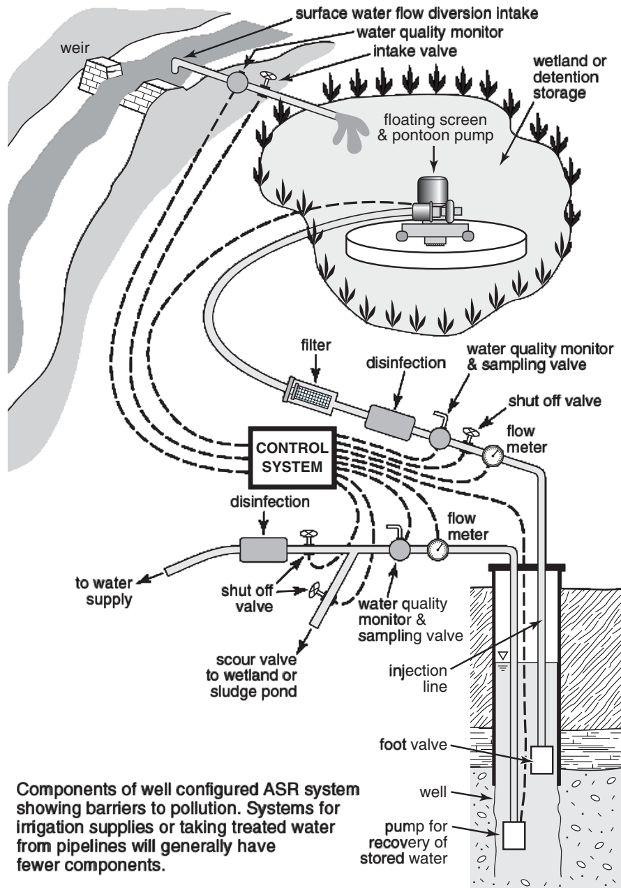
Figure 3. Components of a well-configured stormwater ASR system showing barriers to pollution (from CSIRO Land and Water)
