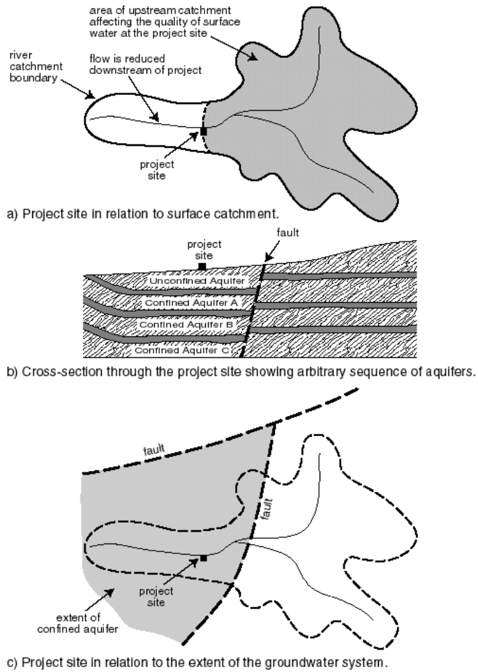
Figure 2. ASR project site in relation to the surface catchment and the groundwater system (from CSIRO Land and Water)
