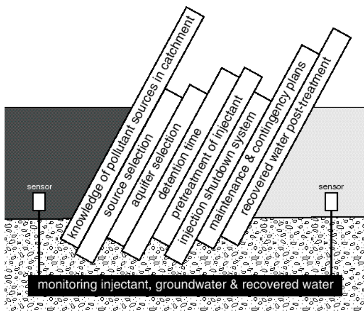
Multiple barriers to protect groundwater and recovered water at ASR projects.
