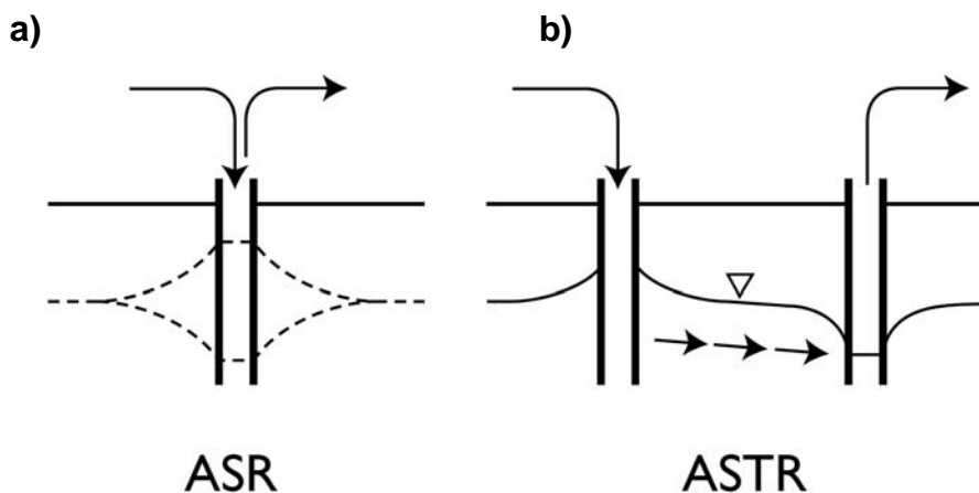
Figure 1. Cross-section diagram of ASR and ASTR (a) ASR by stormwater injection in winter, recovery in summer (b) ASTR where the recovered water has had a guaranteed residence time within the aquifer giving further water quality improvements
